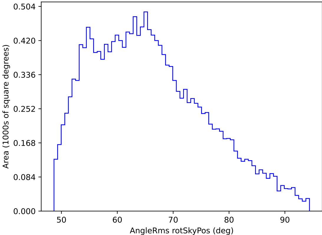
too_elab_r32_d3_gz_v3.4_10yrs WFD z band: AngleRms rotSkyPos
