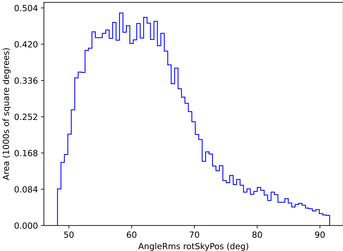
too_elab_r32_d3_gz_v3.4_10yrs WFD y band: AngleRms rotSkyPos
