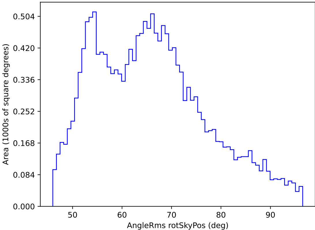
too_elab_r32_d3_gz_v3.4_10yrs WFD r band: AngleRms rotSkyPos
