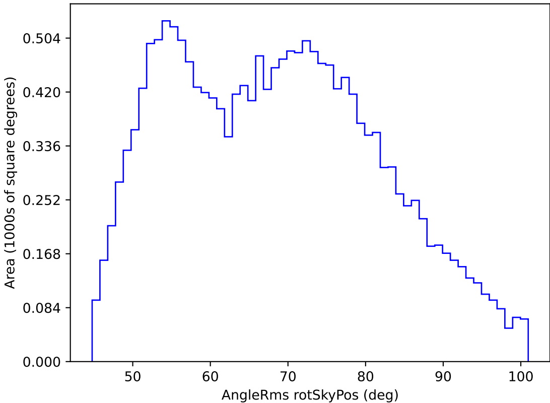
too_elab_r32_d3_gz_v3.4_10yrs WFD g band: AngleRms rotSkyPos
