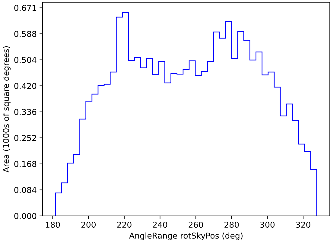
too_elab_r32_d3_gz_v3.4_10yrs WFD u band: AngleRange rotSkyPos
