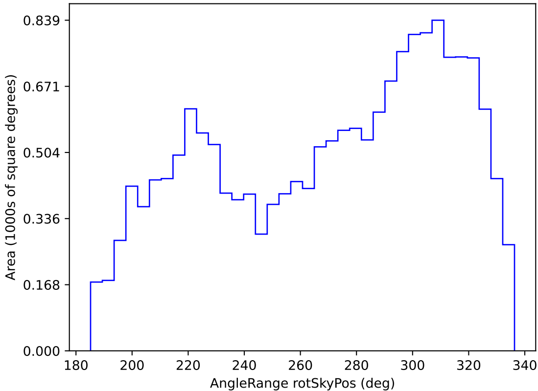
too_elab_r32_d3_gz_v3.4_10yrs WFD g band: AngleRange rotSkyPos
