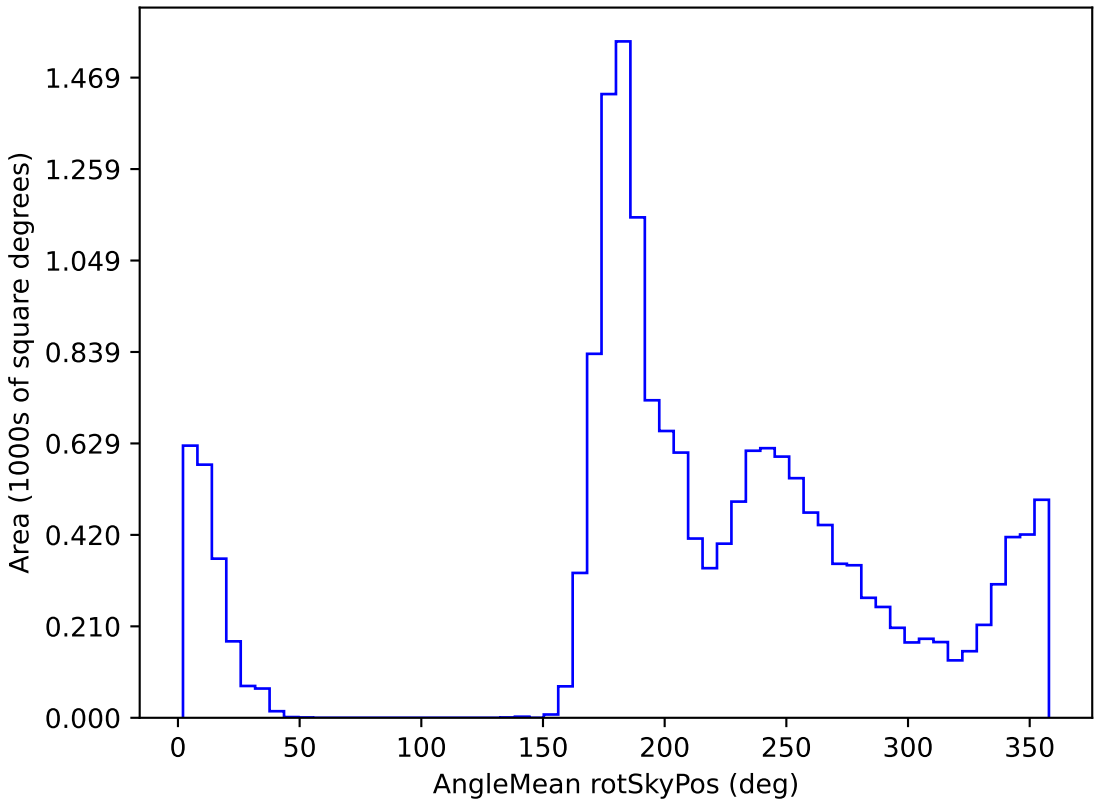
too_elab_r32_d3_gz_v3.4_10yrs WFD z band: AngleMean rotSkyPos
