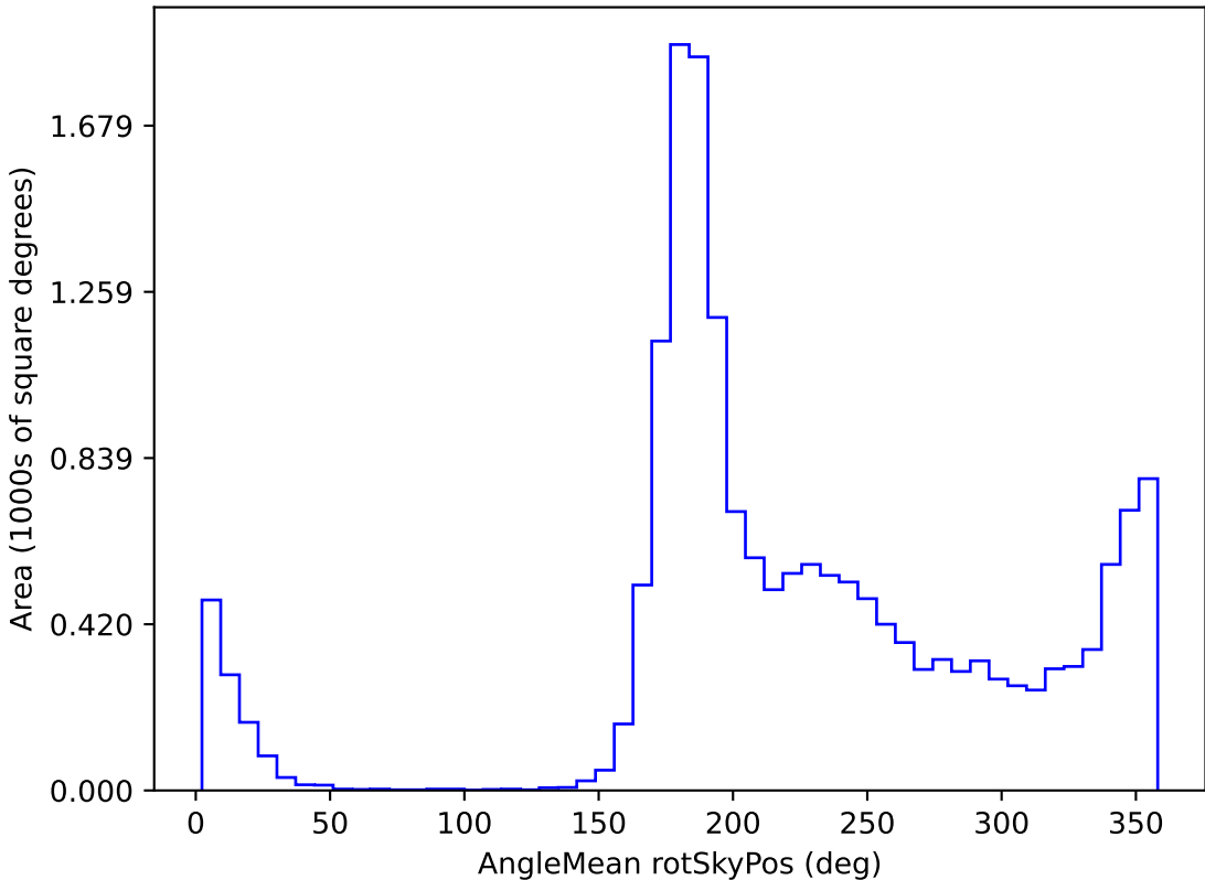
too_elab_r32_d3_gz_v3.4_10yrs WFD u band: AngleMean rotSkyPos
