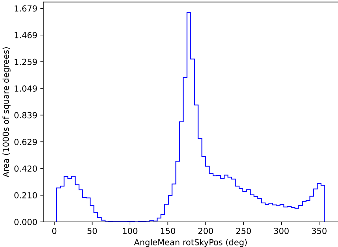
too_elab_r32_d3_gz_v3.4_10yrs WFD g band: AngleMean rotSkyPos
