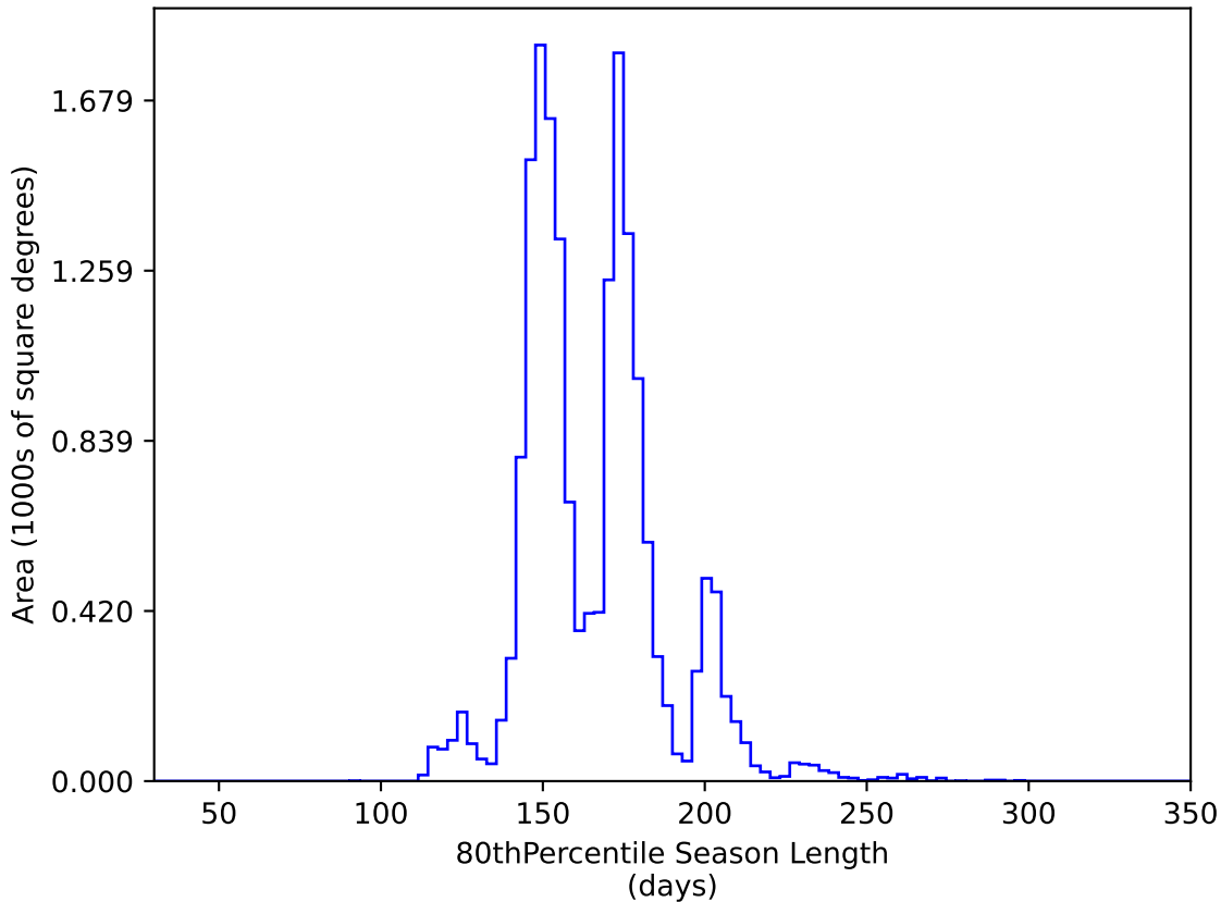
too_elab_r32_d3_gz_v3.4_10yrs WFD y band: 80thPercentile Season Length
