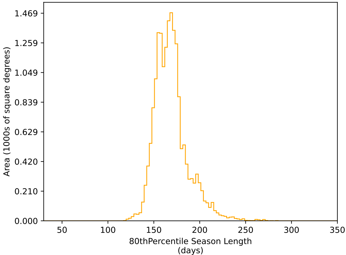
too_elab_r32_d3_gz_v3.4_10yrs WFD r band: 80thPercentile Season Length
