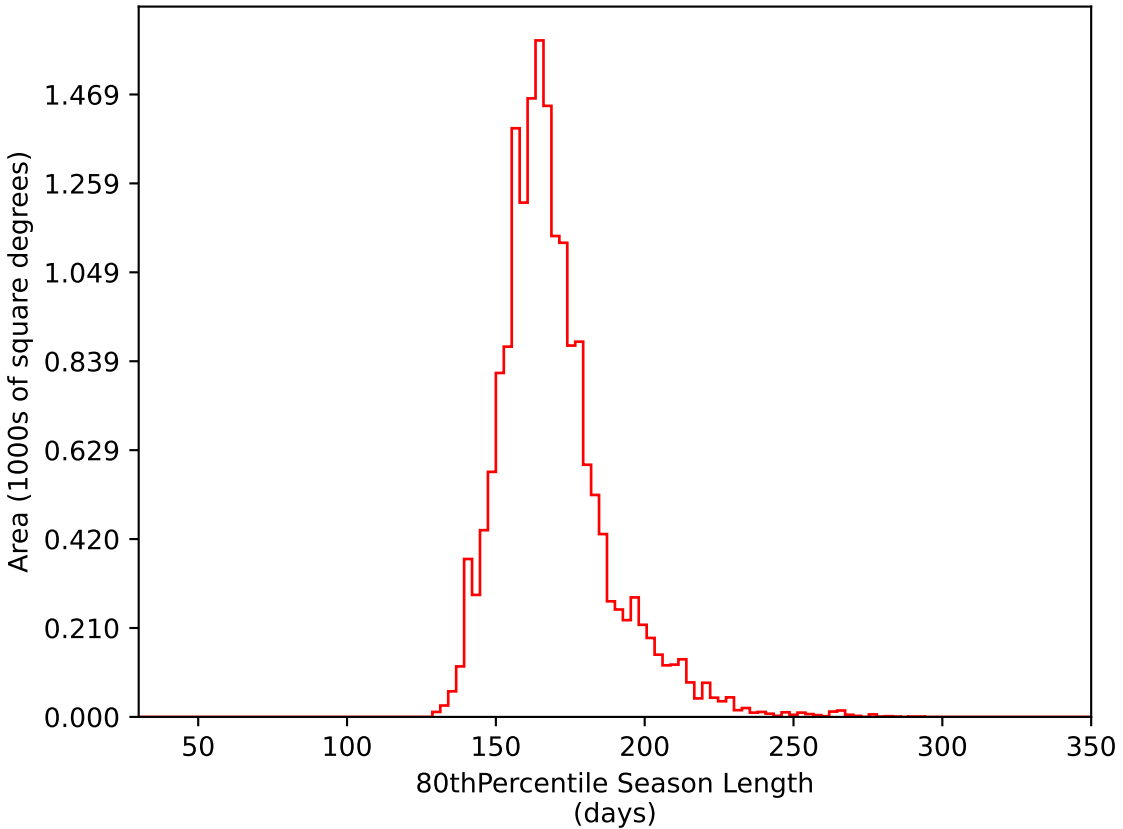
too_elab_r32_d3_gz_v3.4_10yrs WFD i band: 80thPercentile Season Length
