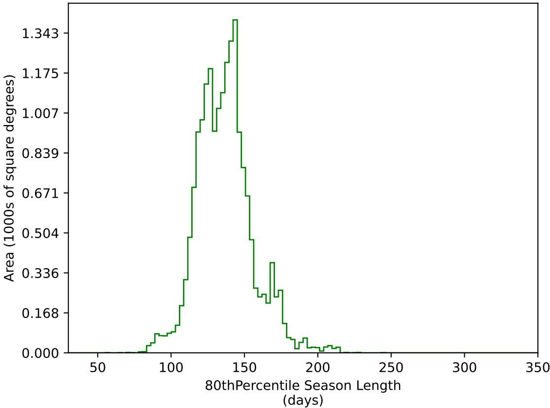
too_elab_r32_d3_gz_v3.4_10yrs WFD g band: 80thPercentile Season Length
