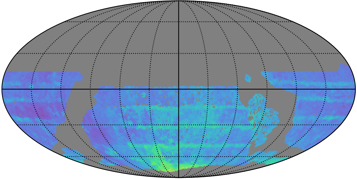
too_elab_r32_d3_gz_v3.4_10yrs WFD all bands: 80thPercentile Season Length
