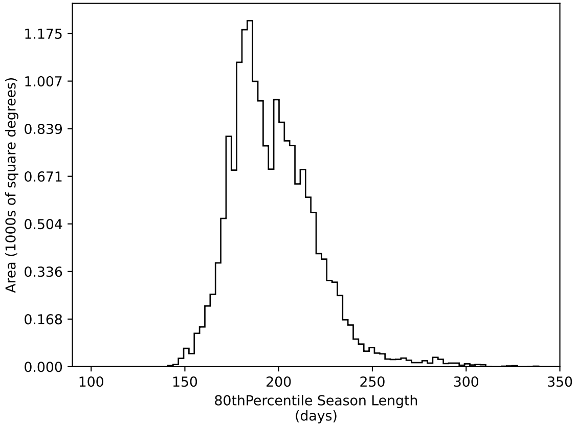
too_elab_r32_d3_gz_v3.4_10yrs WFD all bands: 80thPercentile Season Length
