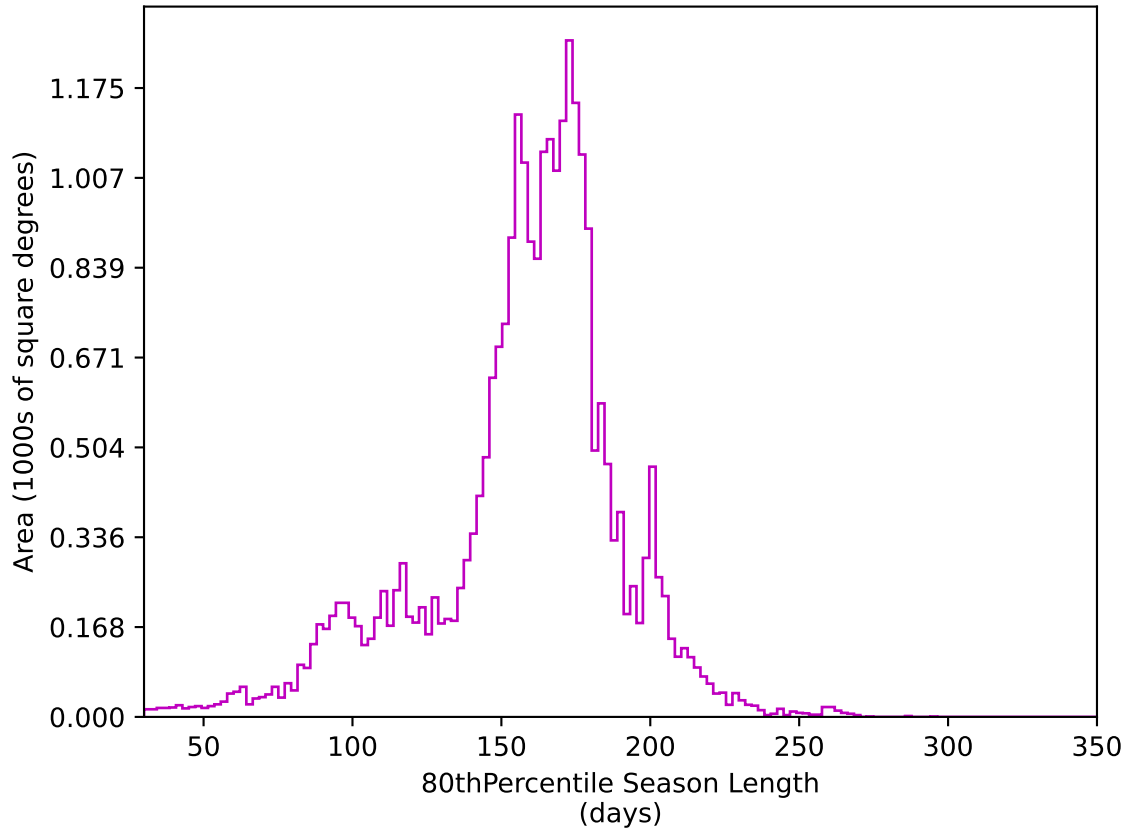
too_elab_r32_d3_gz_v3.4_10yrs All sky z band: 80thPercentile Season Length
