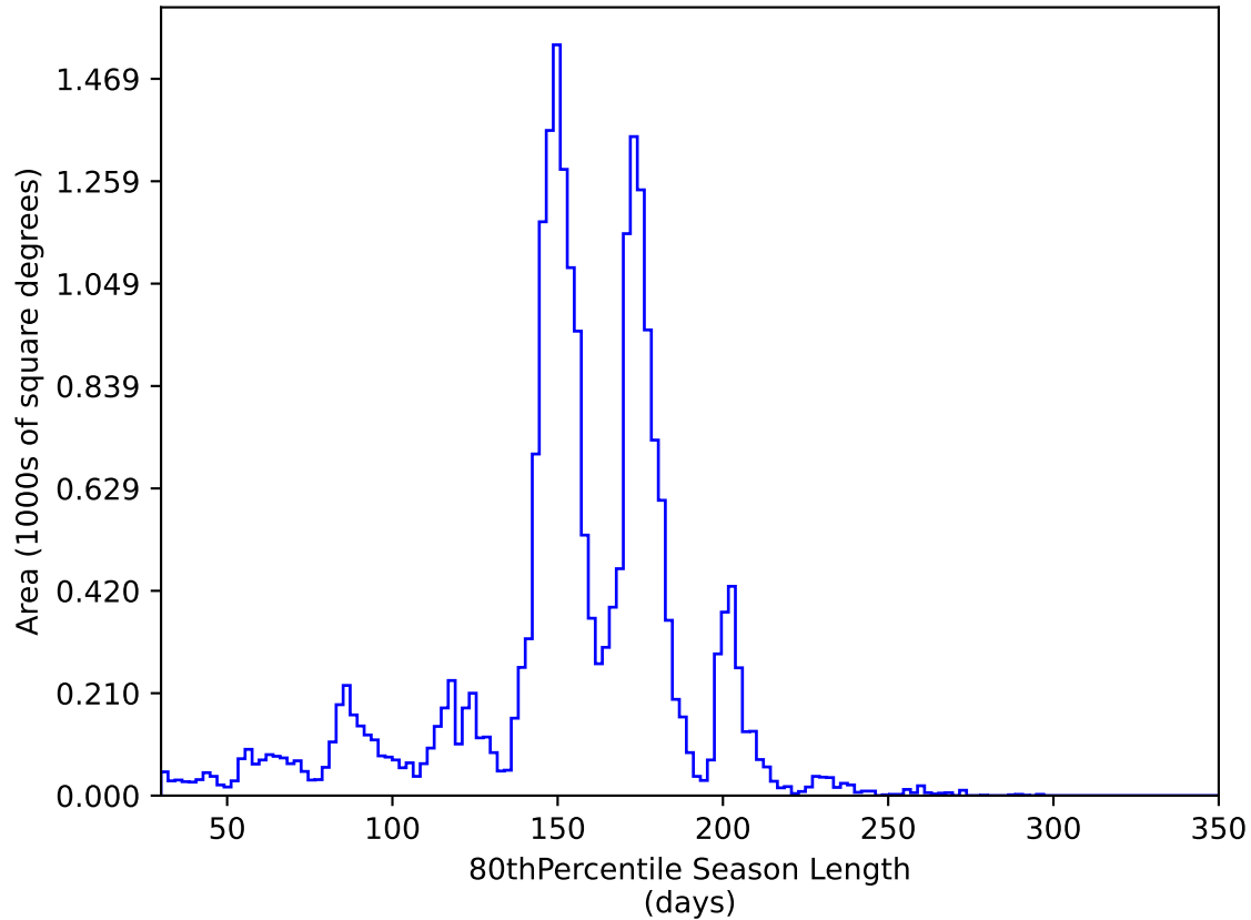
too_elab_r32_d3_gz_v3.4_10yrs All sky y band: 80thPercentile Season Length
