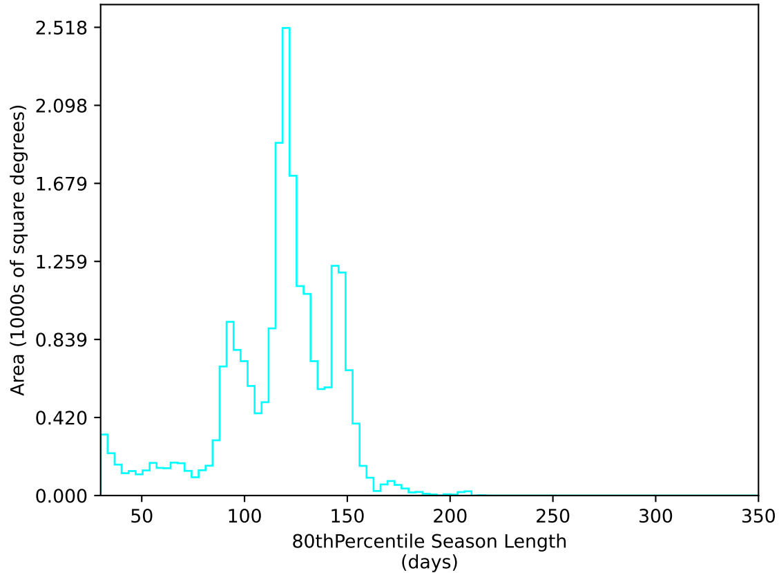
too_elab_r32_d3_gz_v3.4_10yrs All sky u band: 80thPercentile Season Length
