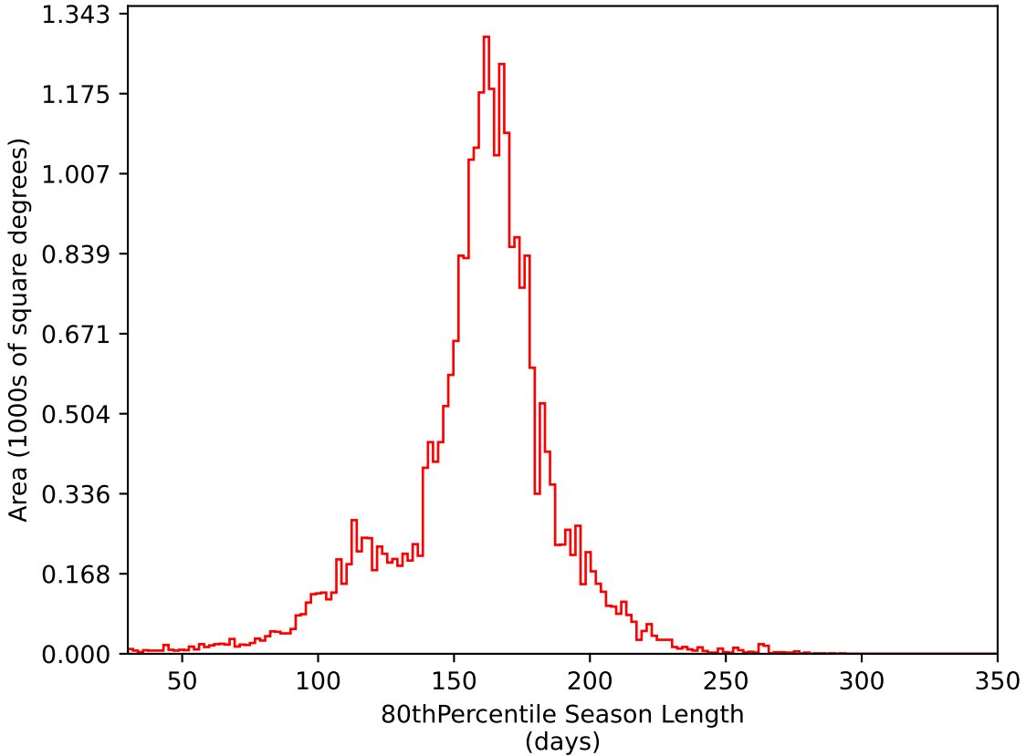
too_elab_r32_d3_gz_v3.4_10yrs All sky i band: 80thPercentile Season Length
