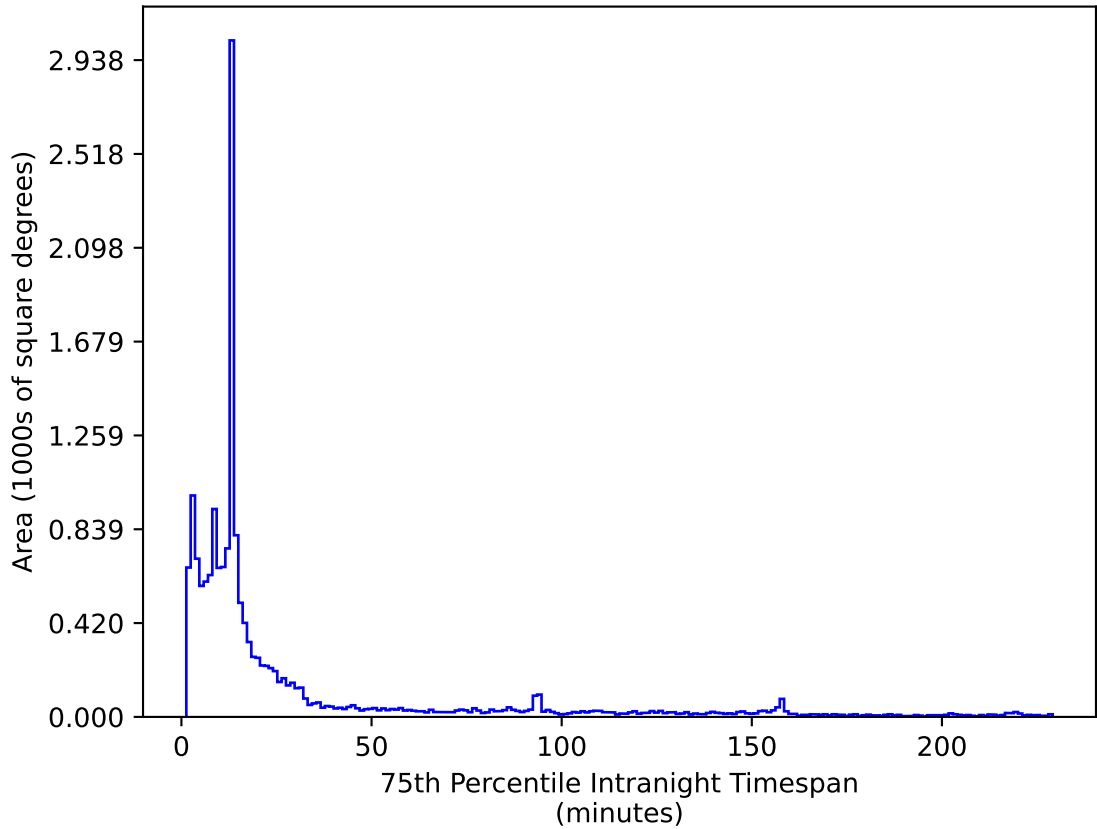
too_elab_r32_d3_gz_v3.4_10yrs WFD z band: 75th Percentile Intranight Timespan
