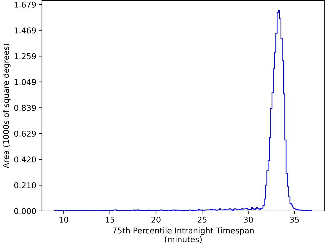
too_elab_r32_d3_gz_v3.4_10yrs WFD ug bands: 75th Percentile Intranight Timespan
