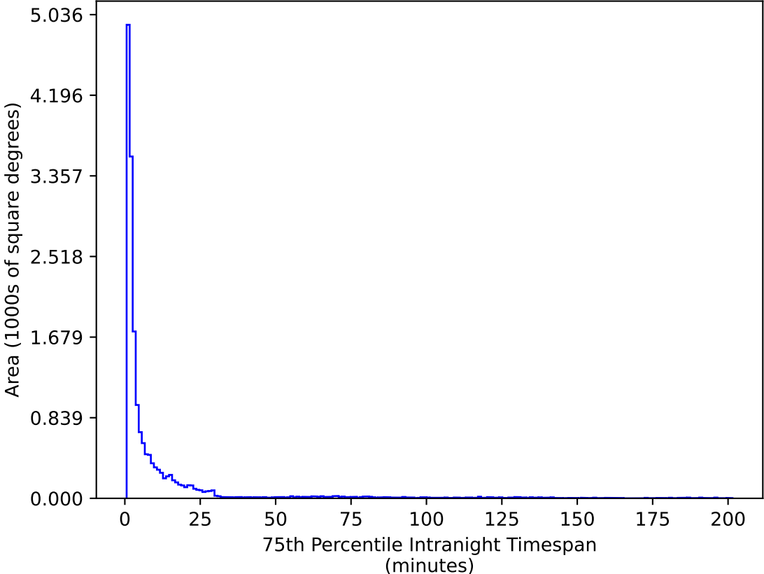
too_elab_r32_d3_gz_v3.4_10yrs WFD u band: 75th Percentile Intranight Timespan
