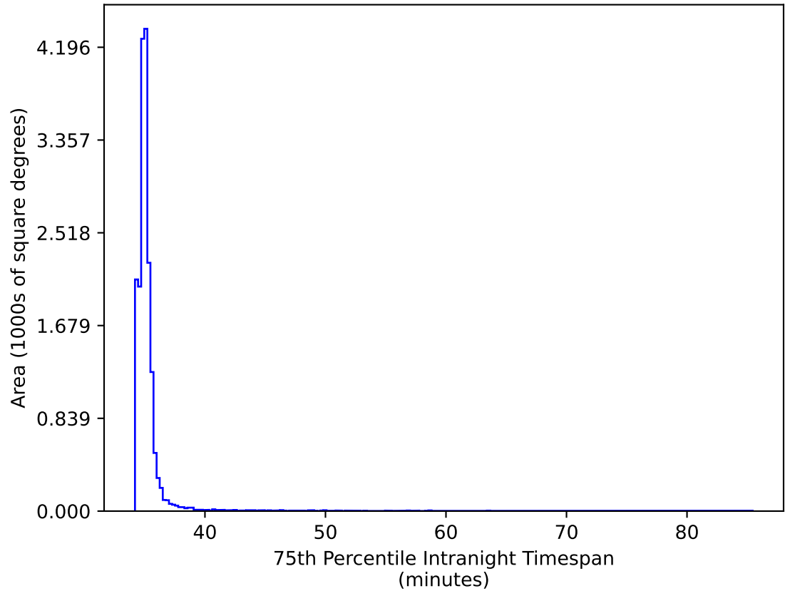
too_elab_r32_d3_gz_v3.4_10yrs WFD ri bands: 75th Percentile Intranight Timespan
