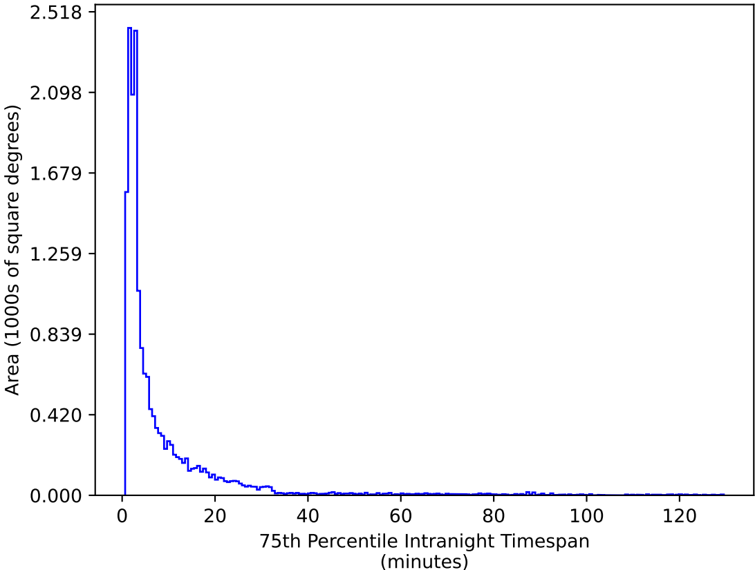
too_elab_r32_d3_gz_v3.4_10yrs WFD g band: 75th Percentile Intranight Timespan
