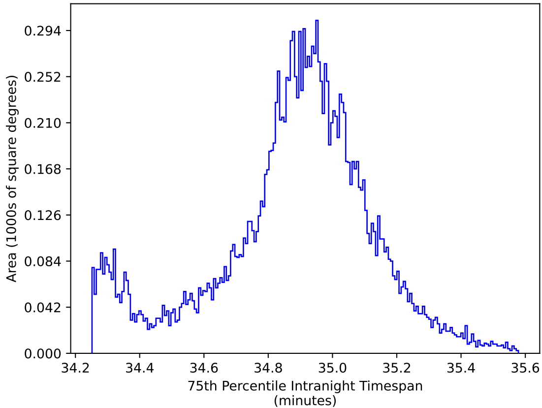
too_elab_r32_d3_gz_v3.4_10yrs WFD all bands: 75th Percentile Intranight Timespan
