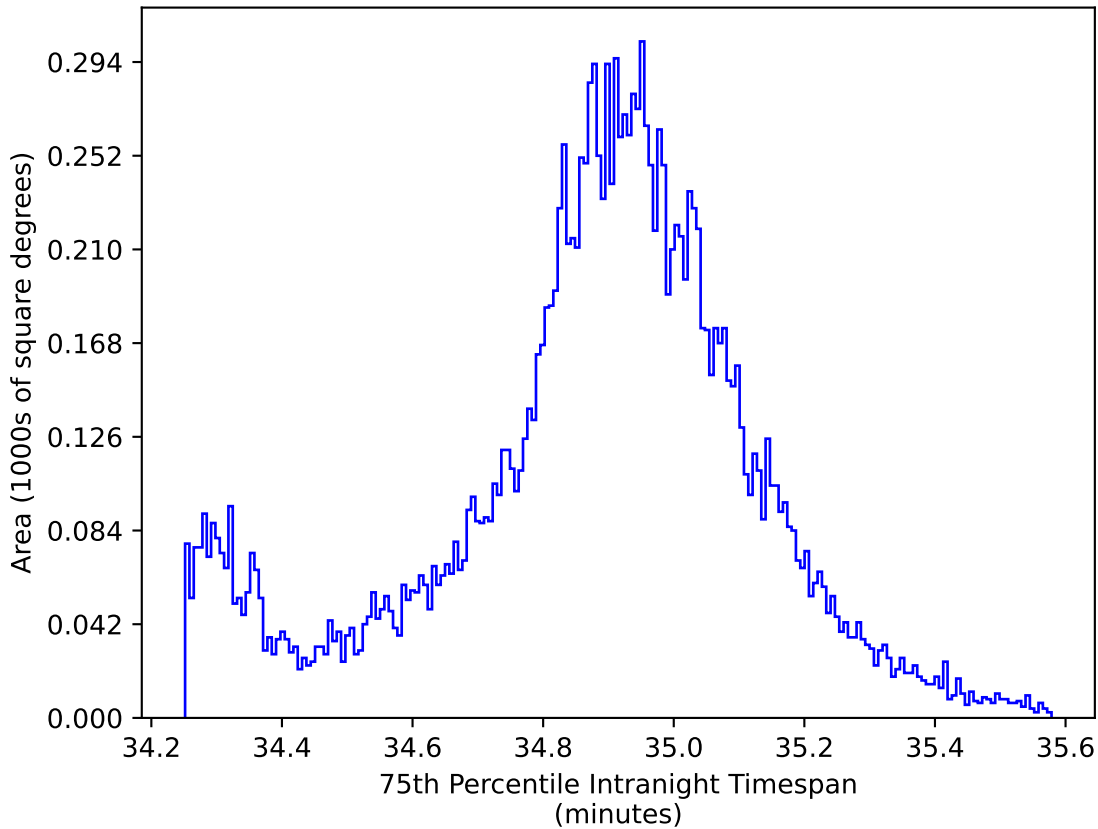
too_elab_r32_d3_gz_v3.4_10yrs WFD: 75th Percentile Intranight Timespan
