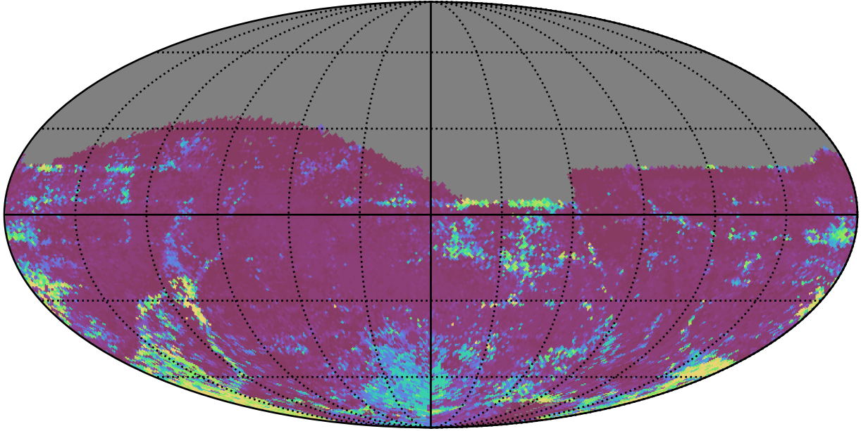
too_elab_r32_d3_gz_v3.4_10yrs All sky z band: 75th Percentile Intranight Timespan
