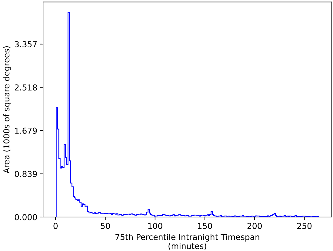
too_elab_r32_d3_gz_v3.4_10yrs All sky z band: 75th Percentile Intranight Timespan
