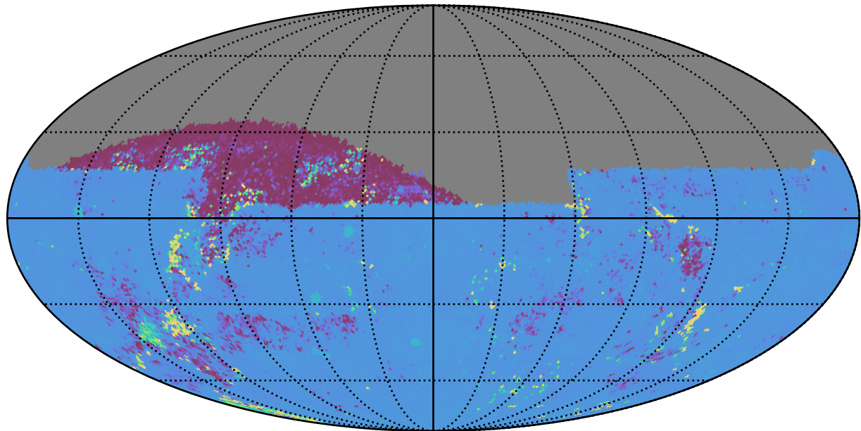
too_elab_r32_d3_gz_v3.4_10yrs All sky ug bands: 75th Percentile Intranight Timespan
