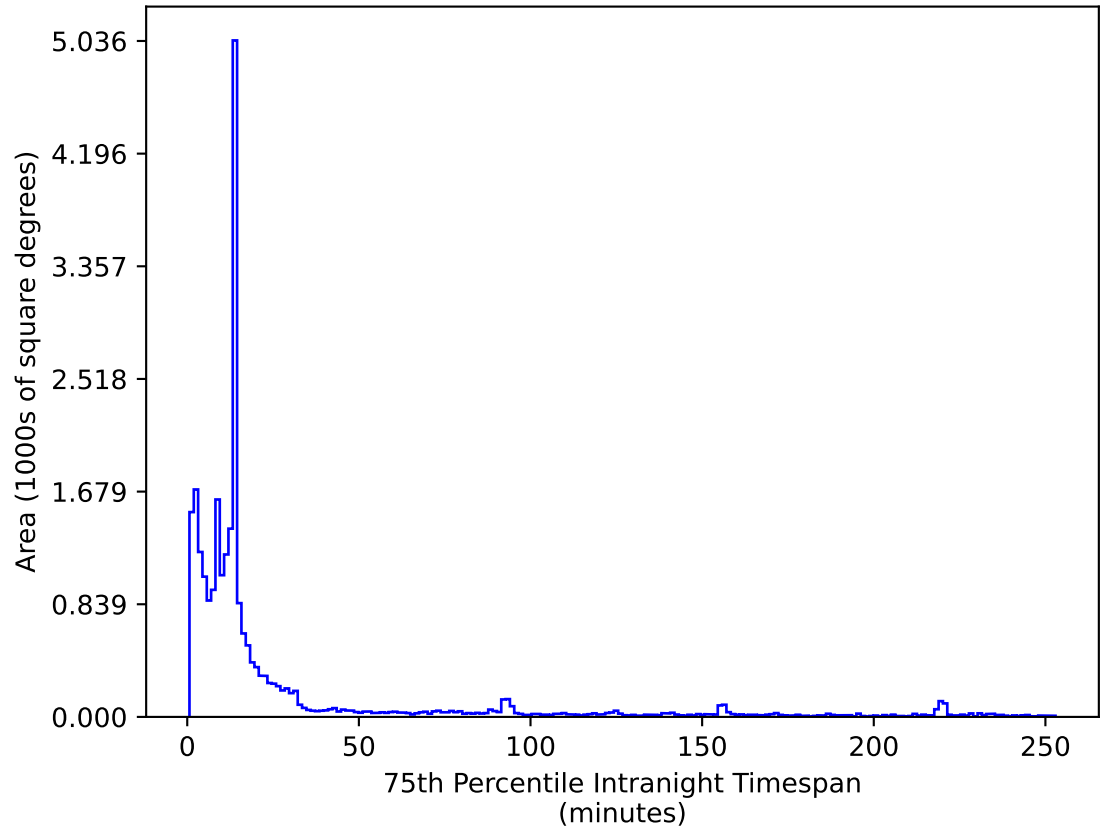
too_elab_r32_d3_gz_v3.4_10yrs All sky i_band: 75th Percentile Intranight Timespan
