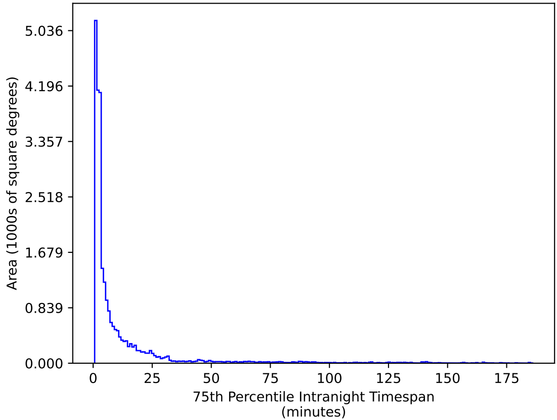
too_elab_r32_d3_gz_v3.4_10yrs All sky g band: 75th Percentile Intranight Timespan
