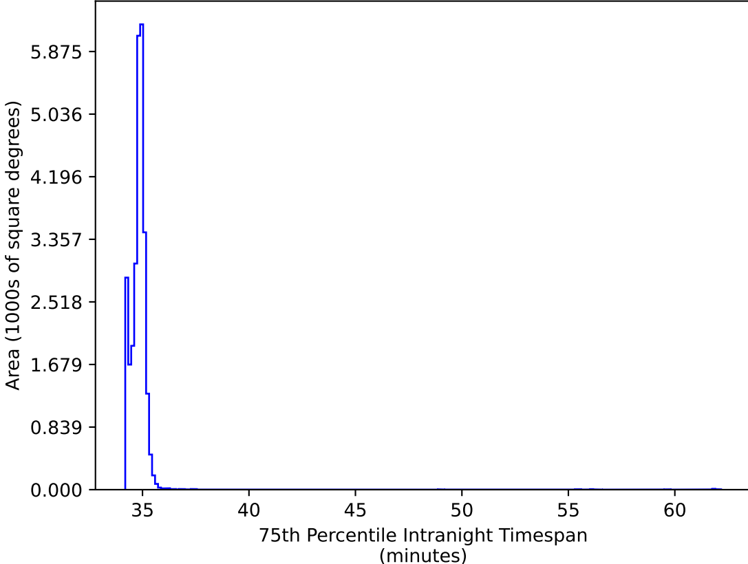
too_elab_r32_d3_gz_v3.4_10yrs All sky all bands: 75th Percentile Intranight Timespan
