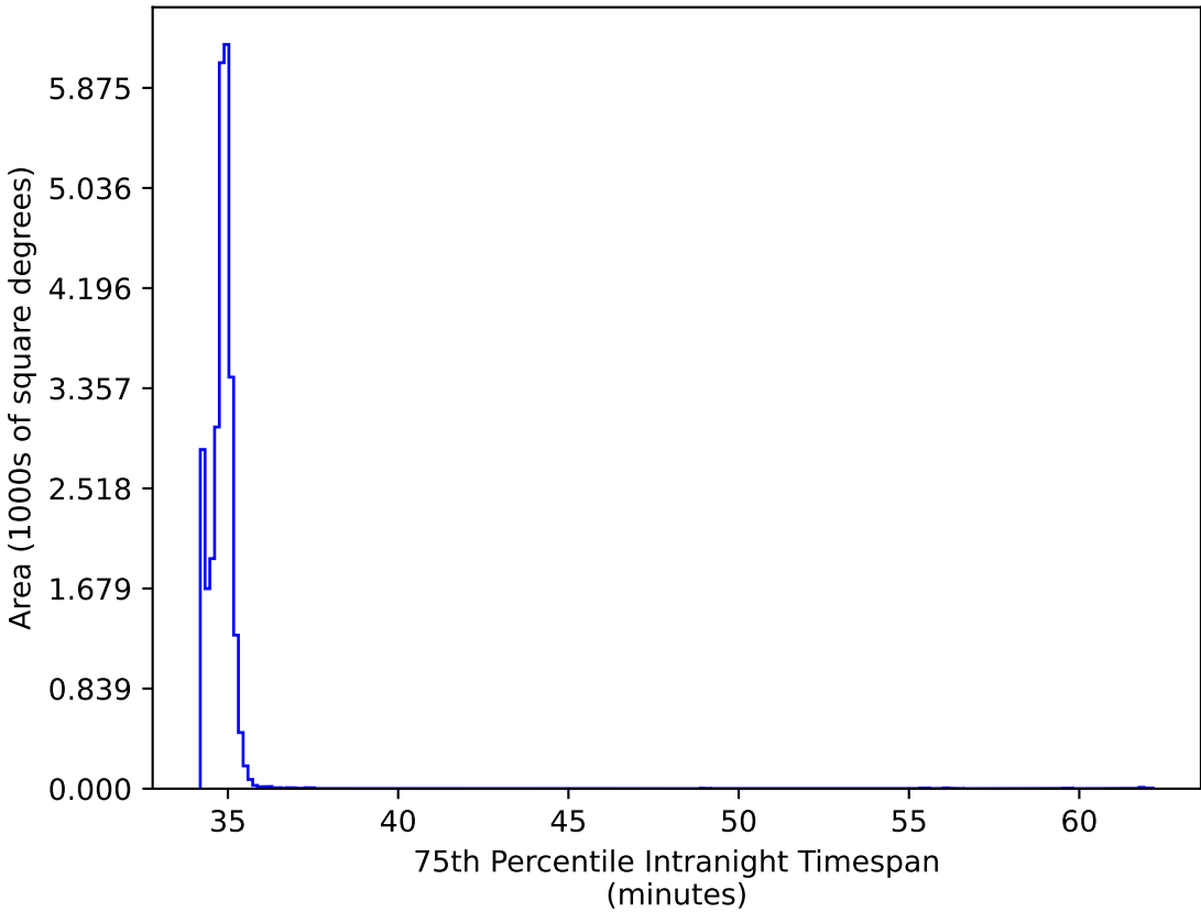
too_elab_r32_d3_gz_v3.4_10yrs All sky: 75th Percentile Intranight Timespan
