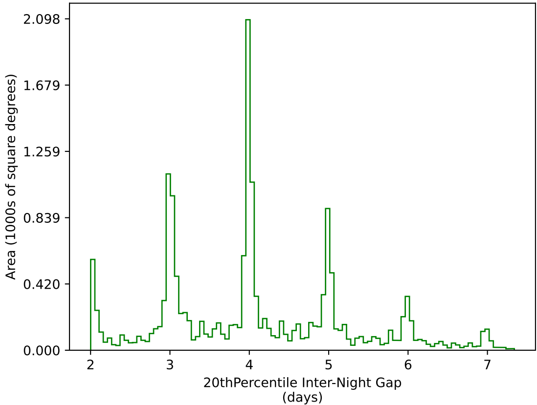
too_elab_r32_d3_gz_v3.4_10yrs WFD g band: 20thPercentile Inter-Night Gap
