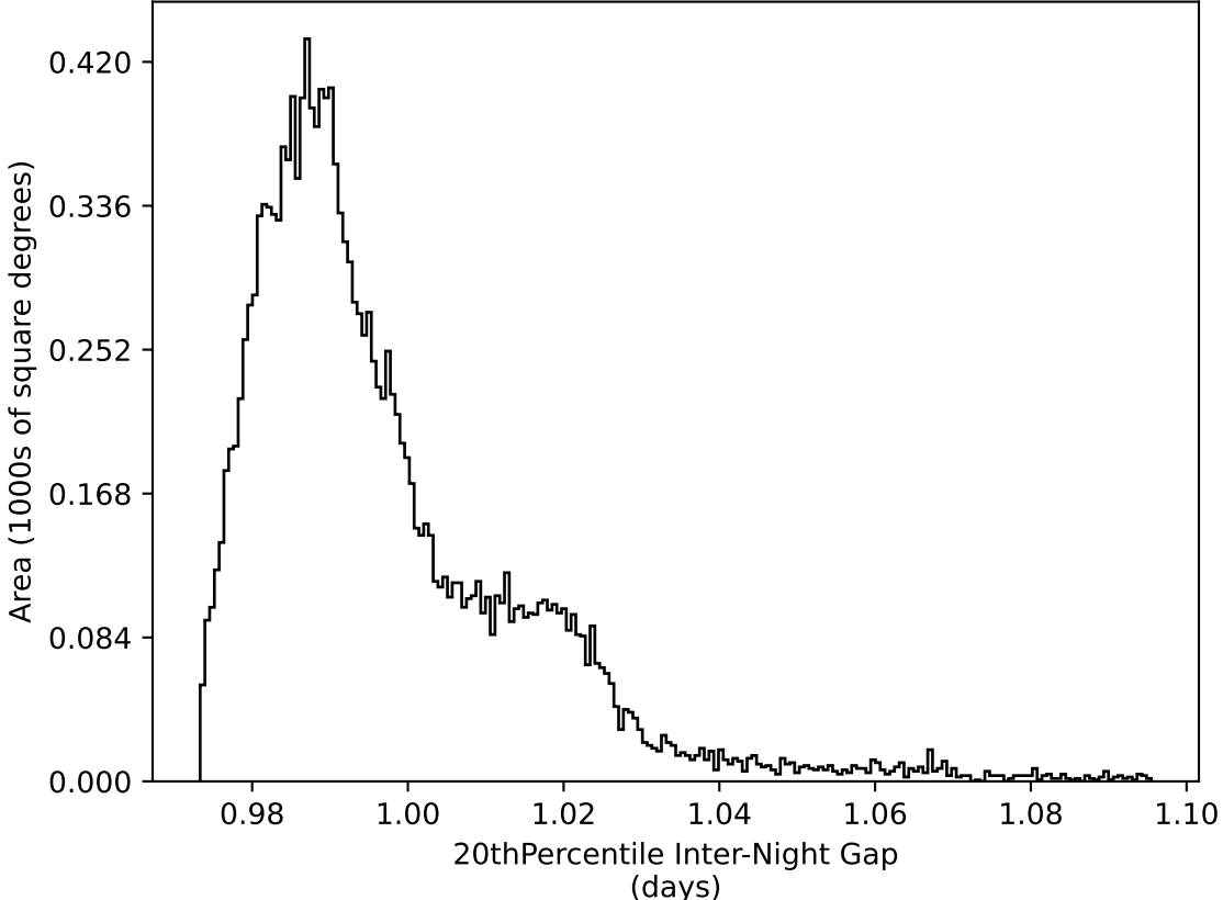
too_elab_r32_d3_gz_v3.4_10yrs WFD all bands: 20thPercentile Inter-Night Gap
