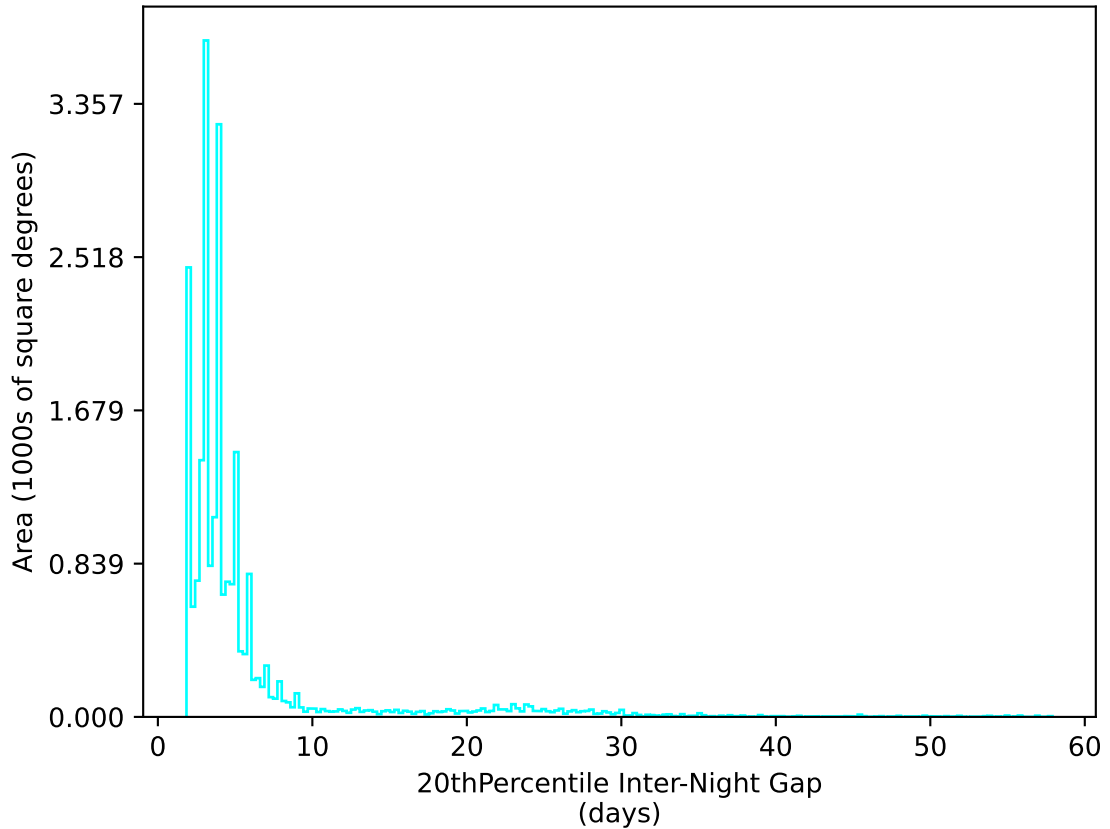
too_elab_r32_d3_gz_v3.4_10yrs All sky u band: 20thPercentile Inter-Night Gap
