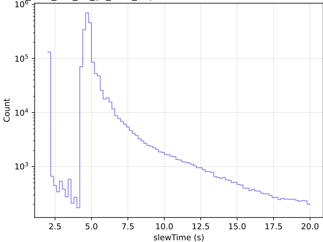
too_elab_r32_d3_gz_v3.4_10yrs All visits: Zoom Slew Time Histogram
