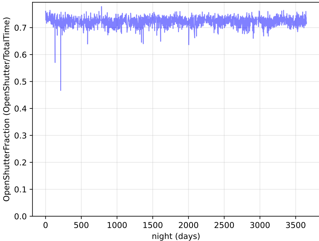
too_elab_r32_d3_gz_v3.4_10yrs : OpenShutterFraction
