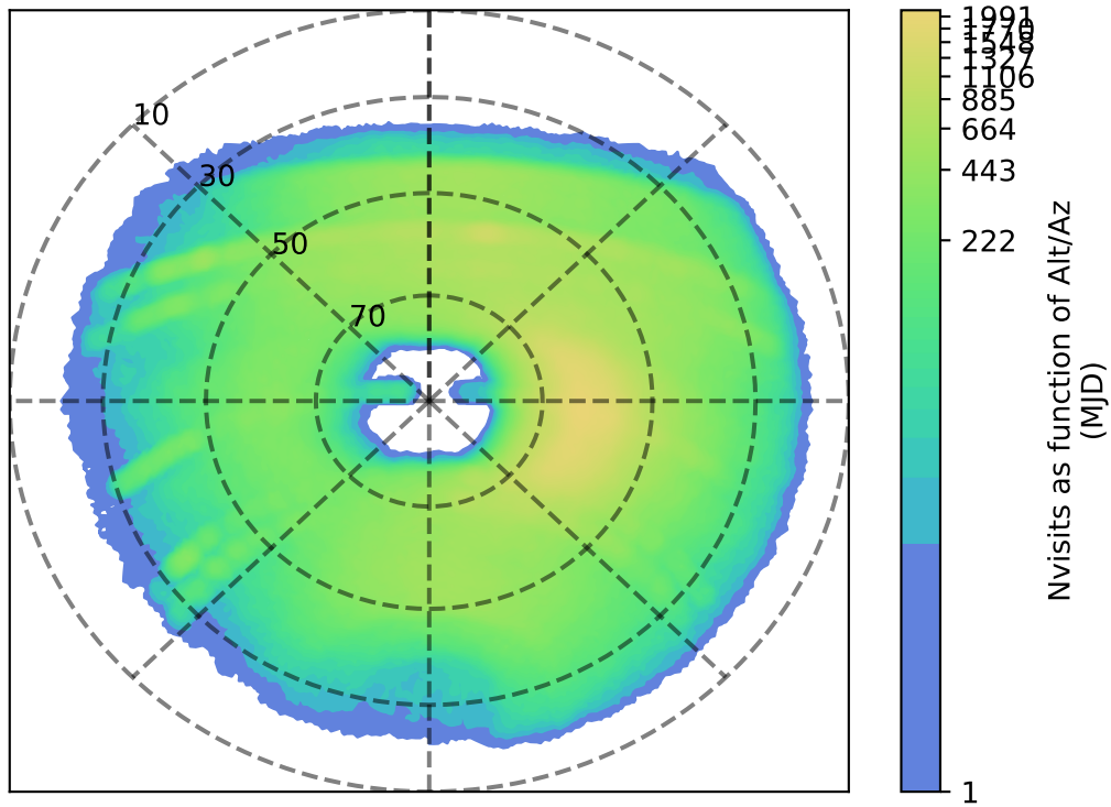
too_elab_r32_d3_gz_v3.4_10yrs y: Nvisits as function of Alt/Az
