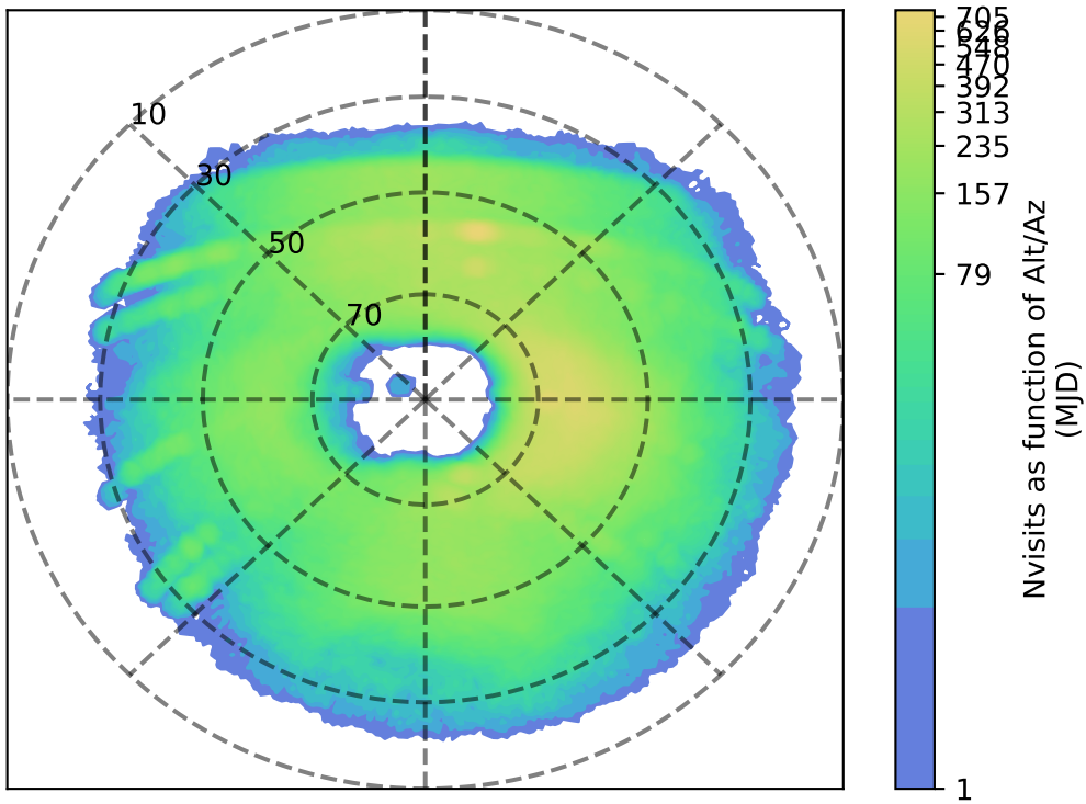
too_elab_r32_d3_gz_v3.4_10yrs u: Nvisits as function of Alt/Az
