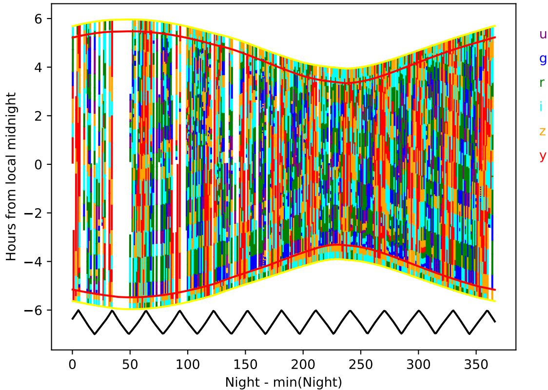
too_elab_r32_d3_gz_v3.4_10yrs year 6-7: Hourglass
