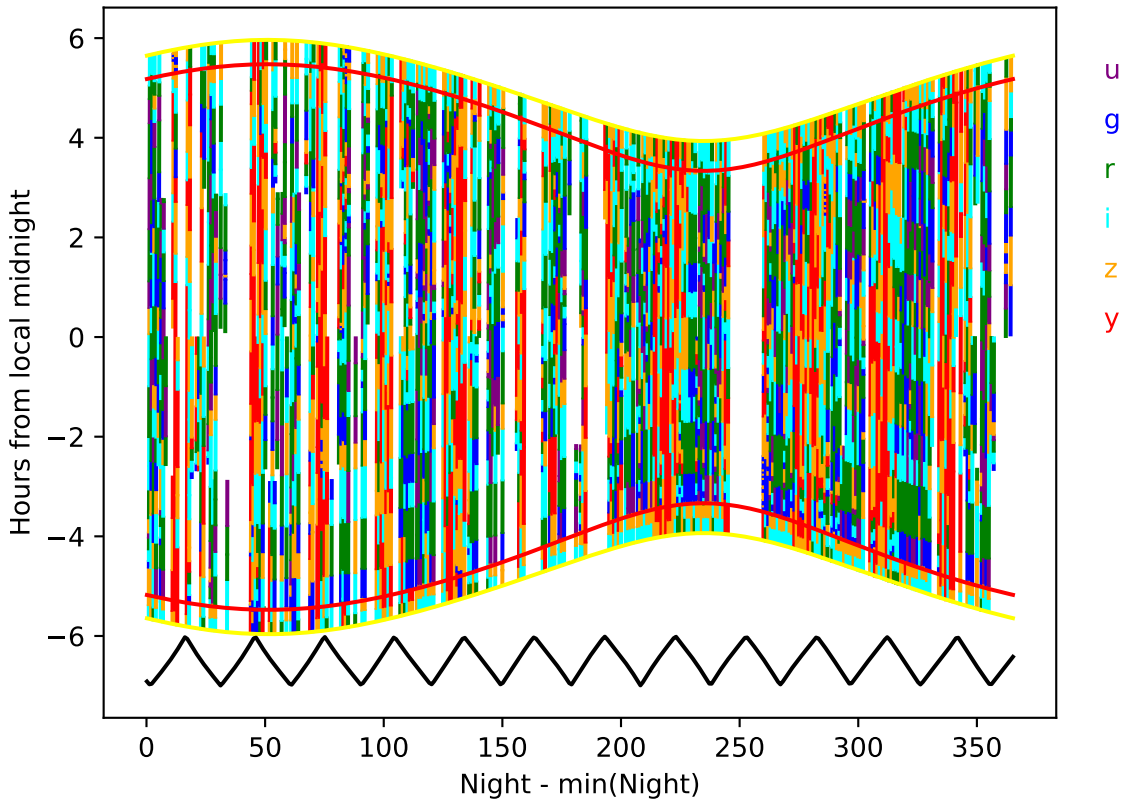
too_elab_r32_d3_gz_v3.4_10yrs year 5-6: Hourglass
