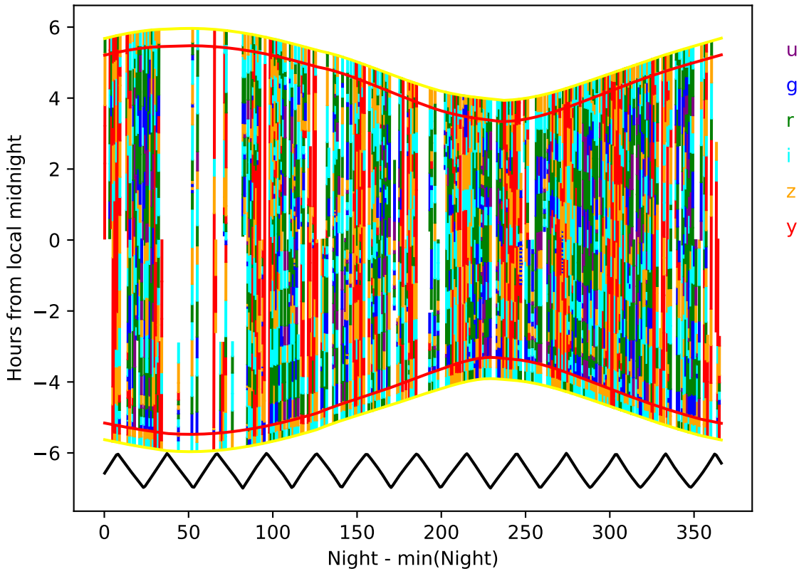
too_elab_r32_d3_gz_v3.4_10yrs year 3-4: Hourglass
