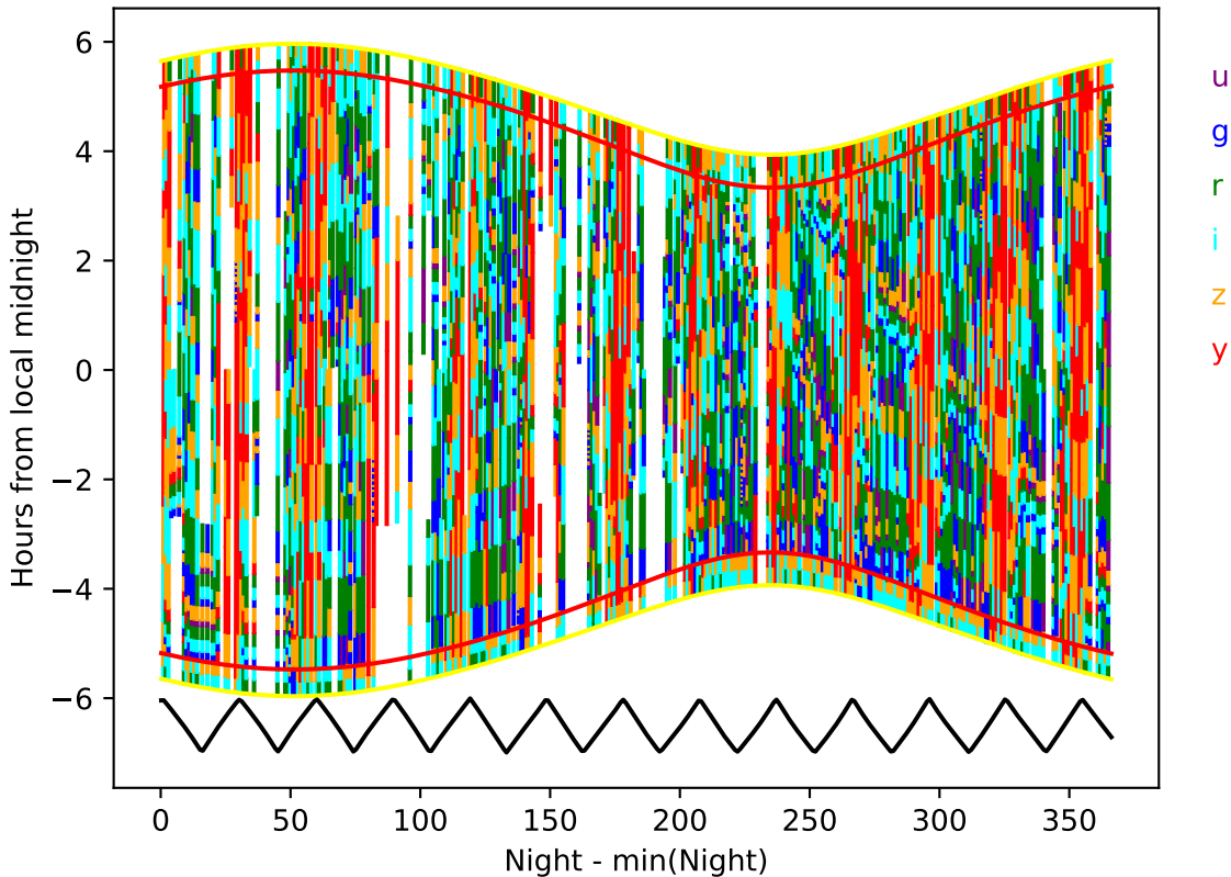
too_elab_r32_d3_gz_v3.4_10yrs year 1-2: Hourglass
