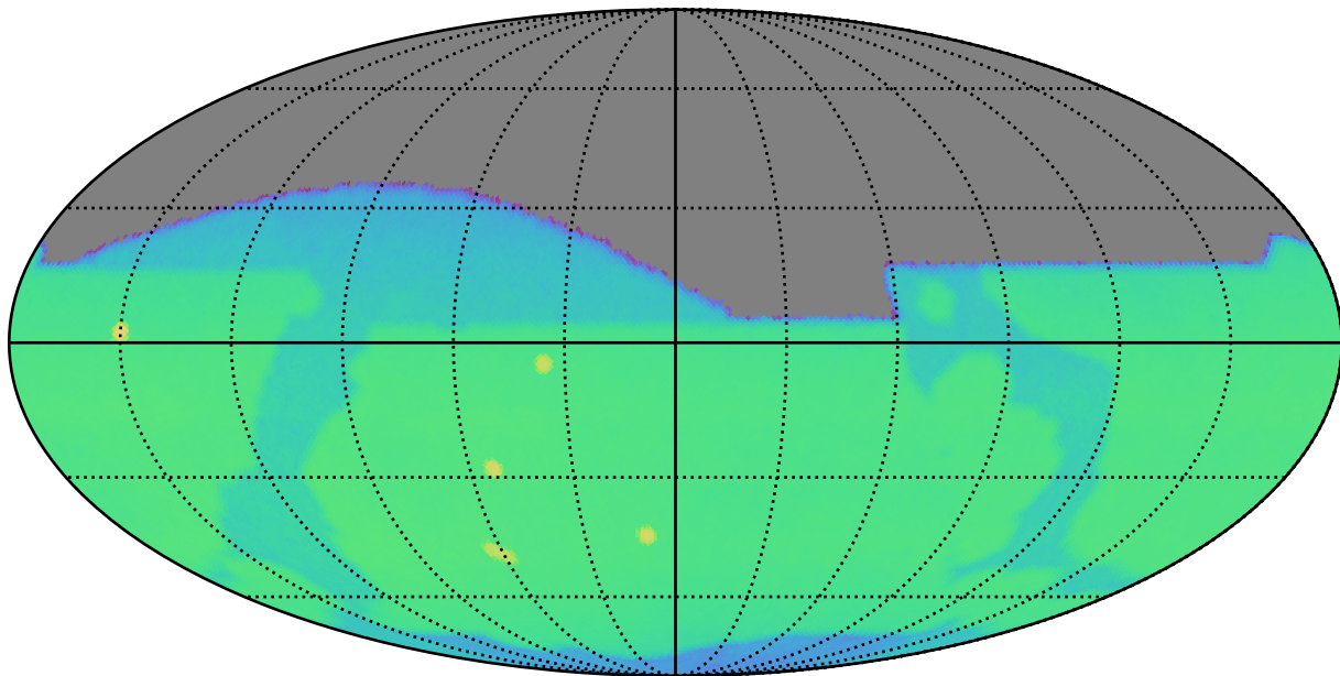
too_elab_r32_d3_gz_v3.4_10yrs i: CoaddM5
