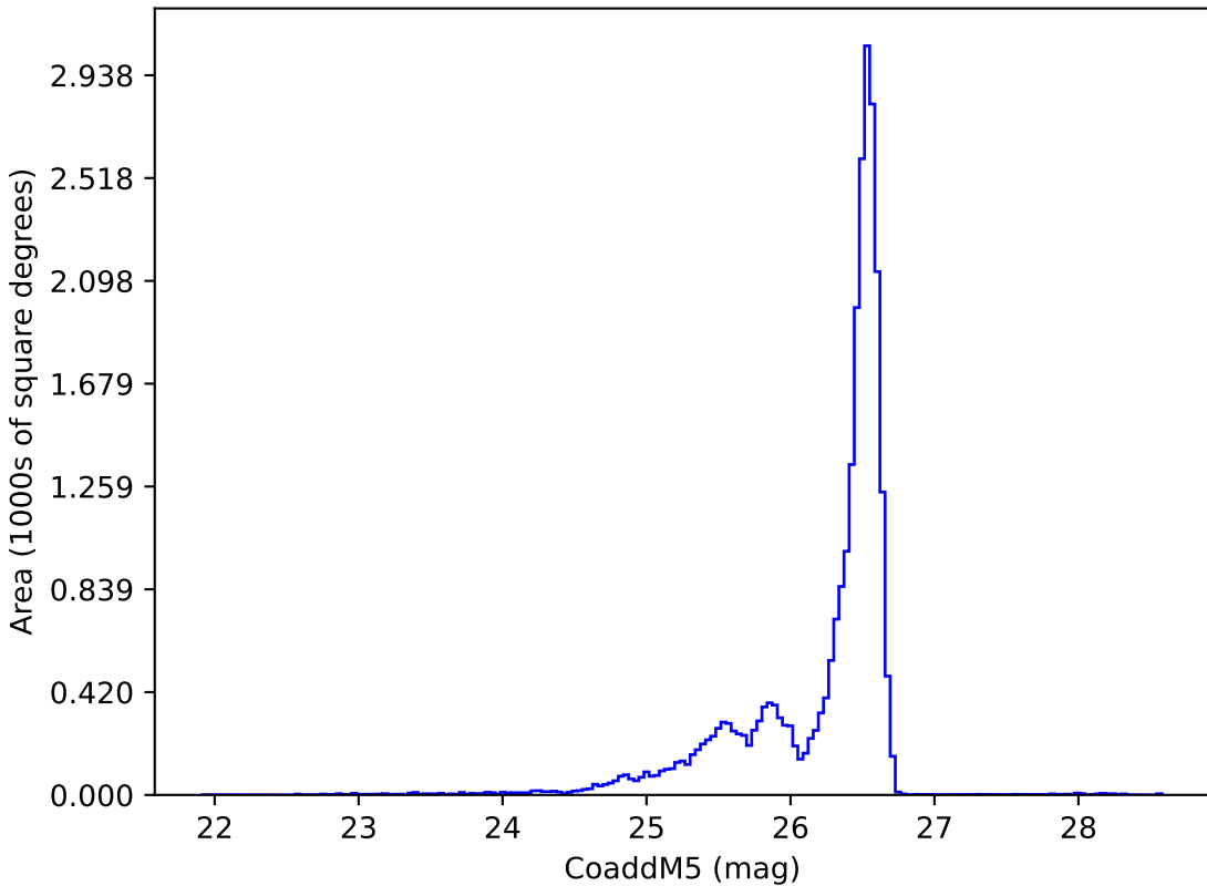
too_elab_r32_d3_gz_v3.4_10yrs i: CoaddM5
