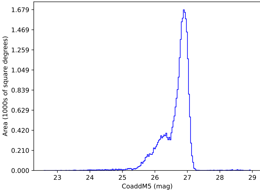
too_elab_r32_d3_gz_v3.4_10yrs g: CoaddM5
