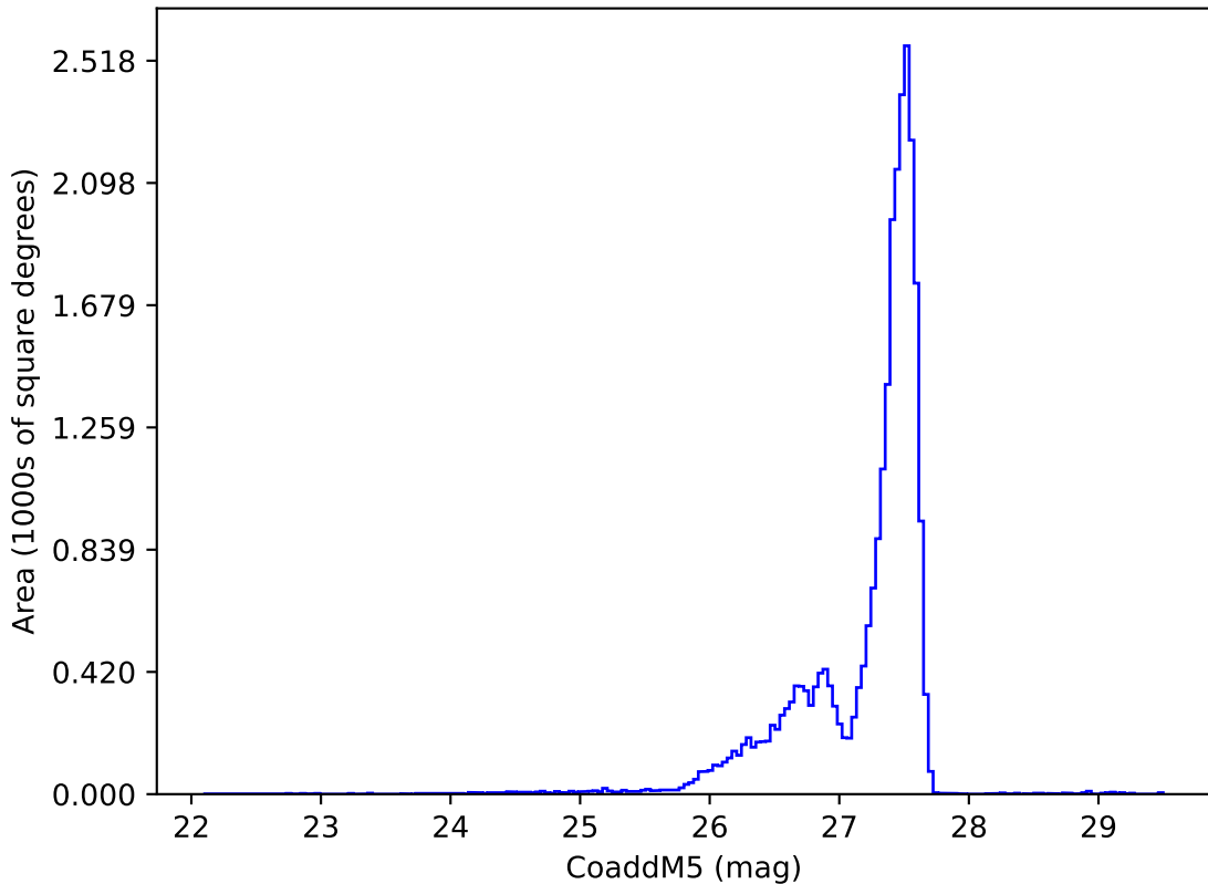
too_elab_r32_d3_gz_v3.4_10yrs : CoaddM5
