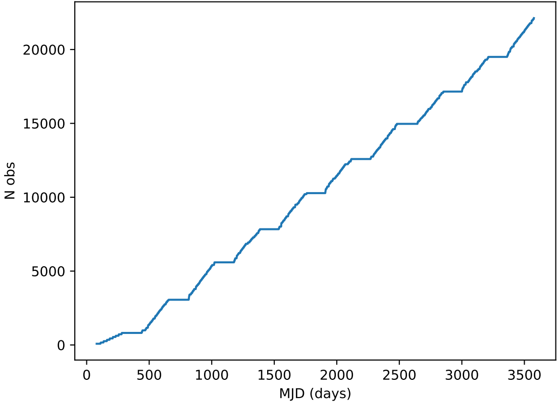
too_elab_r32_d3_gz_v3.4_10yrs all bands: DD:XMM_LSS Cumulative NVisits
