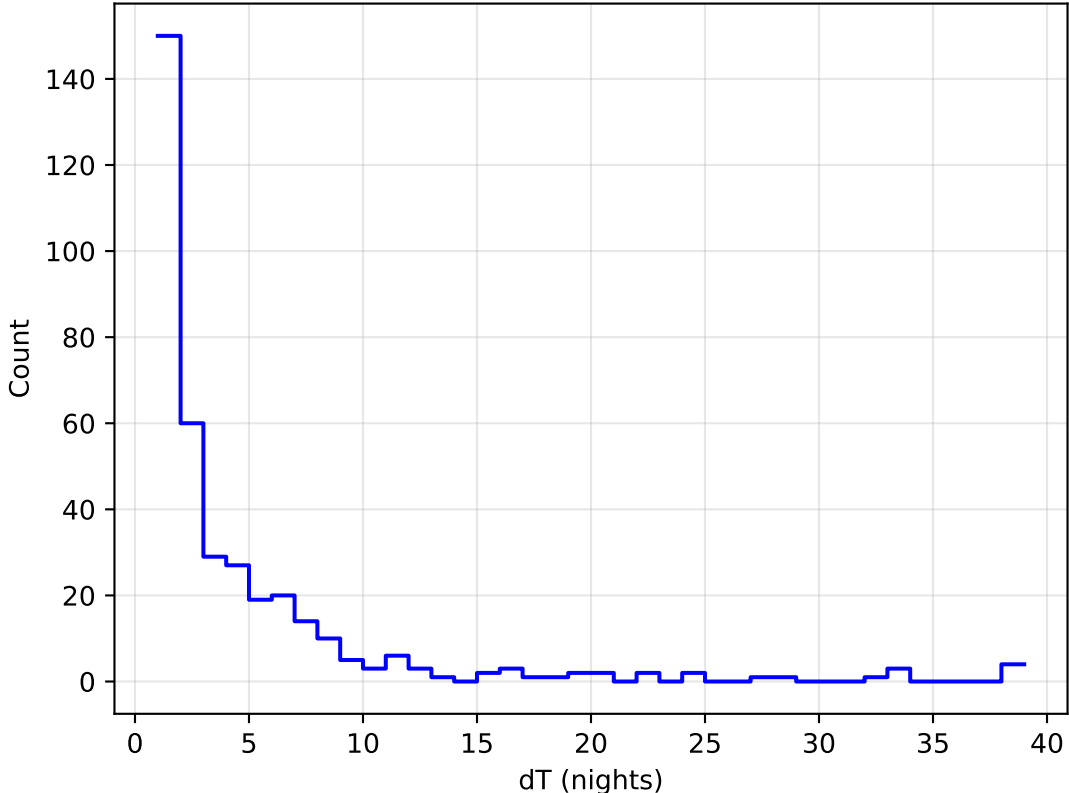
too_elab_r32_d3_gz_v3.4_10yrs all bands: DD:WFD Delta Nights Histogram
